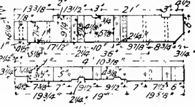
Figs. 1964-65. Draft-timbers.
